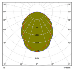
ST30Y44P4X15-50 (1 Strip)
