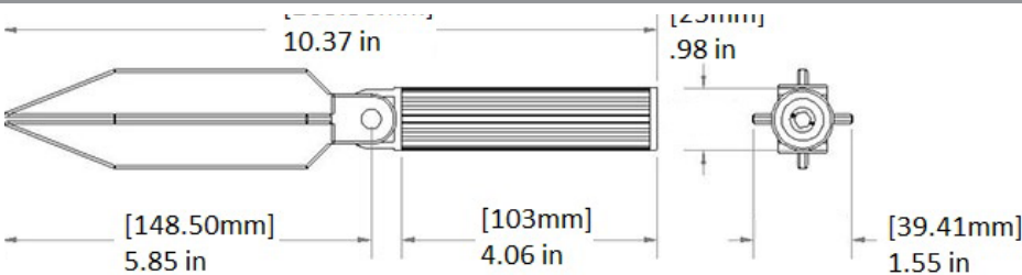
LS25 dimensions for being placed in ground.
