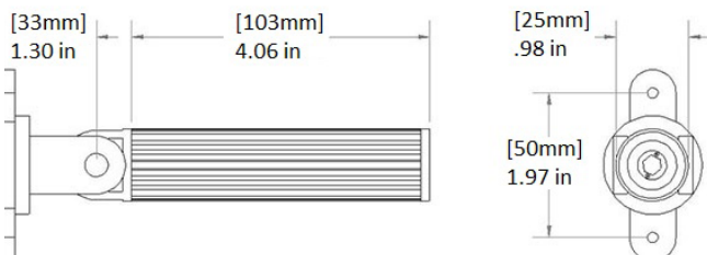
LS25 dimensions for being placed in ground.
